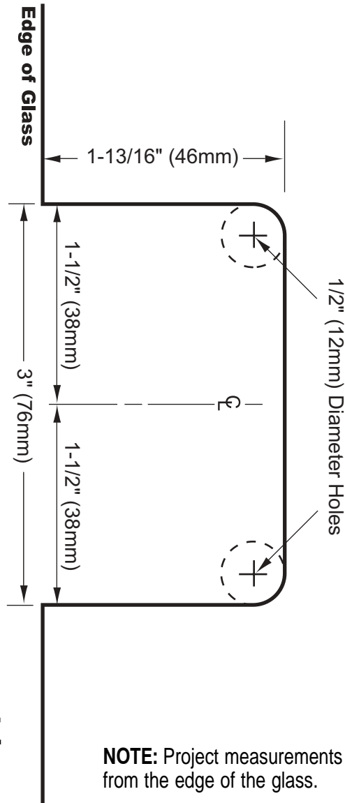
Rectangular Cut-out Option
